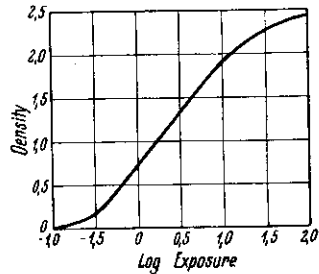
Figure 18. Characteristic curve of a photographic plate.
