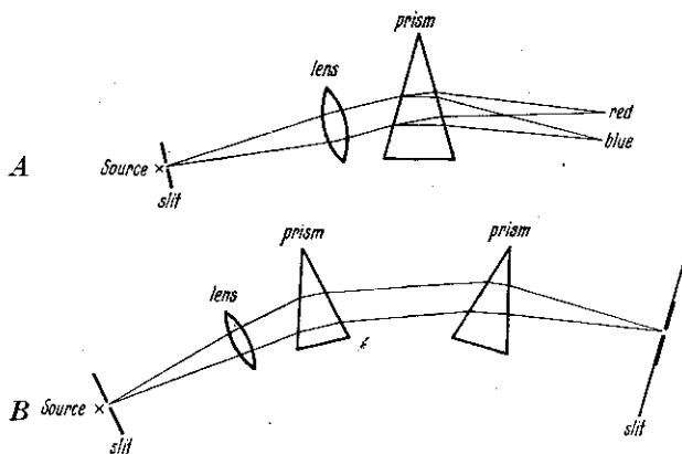
Figure 15. Spectrometers
