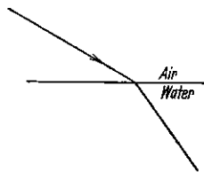
Figure 1. Refraction.
