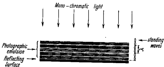
Figure 8. Experiment showing the wave nature of light.
