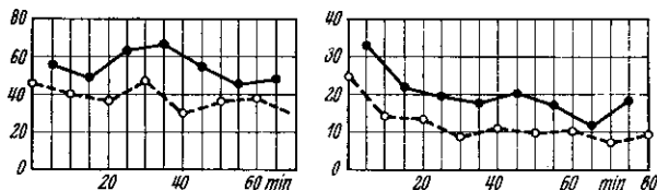
Figure 21. The ordinates are the number of impacts obtained per 5 minute interval, when the counter is exposed alternately for 5 minutes and shielded from the source of radiation. The source of radiation was at the left the chemical reaction K_2Cr_2O_7 + FeSO_4 , at the right a tetanized sartorius muscle of the frog.
