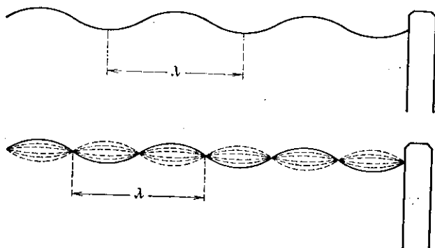
Figure 4. Above: Waves in a rope; below: standing waves in a rope.
