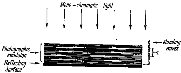
Figure 8. Experiment showing the wave nature of light.
