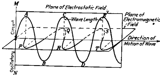
Figure 6. Diagram of an electromagnetic wave.
