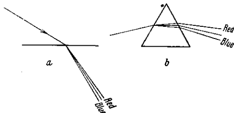
Figure 2. Refraction and Dispersion.
