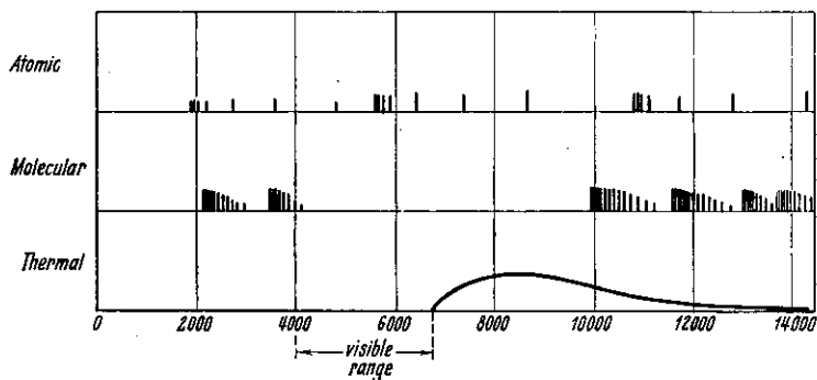
Figure 14. Representation of atomic, molecular, and thermal radiation.
