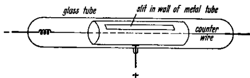
Figure 20. Photoelectric tube counter.
